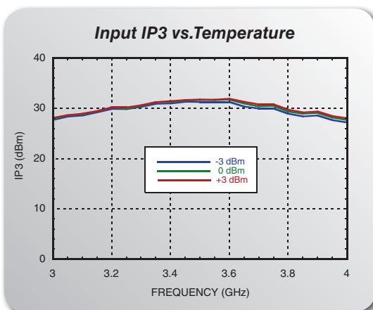
HMC666LP4E High IP3 DBL-BAL Mixer, 3.3 - 3.9 GHz
