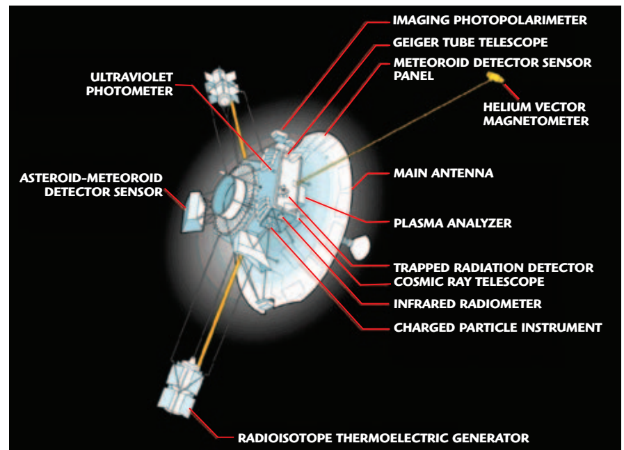
▲ Fig. 3 Design of Pioneer 10 space probe (courtesy of NASA).
